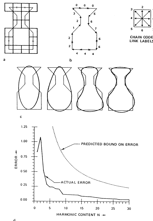
FIG. 1. Properties of the chain code V_1 = 0005676644422123 . (a) Area-quantized image. (b) Chain code of image. (c) 1-, 2-, 3-, and 4-harmonic representations of the chain code V_1 . (d) Actual error and predicted bound on error versus harmonic content.
