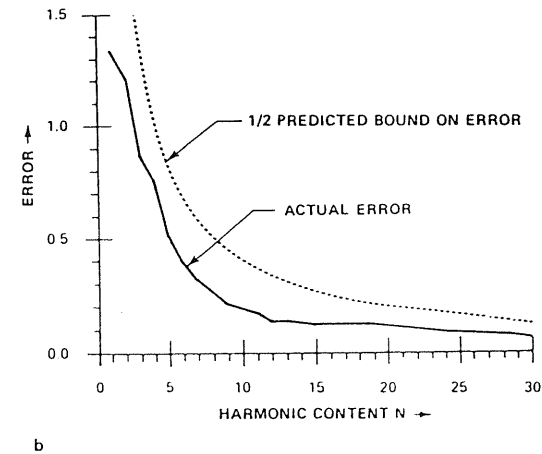
FIG. 2. Properties of the chain code V_2 = 1117220666766644444222 . (a) 1-, 2-, 5-, and 7-harmonic representations of the chain code. (b) Actual error and predicted bound on error versus harmonic content.
