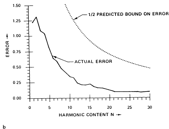
FIG. 4. Properties of the chain code V_4 = 00466026046246532671240224 . (a) 1-, 3-, 7-, and 15-harmonic representations of the chain code. (b) Actual error and predicted bound on error versus harmonic content.
